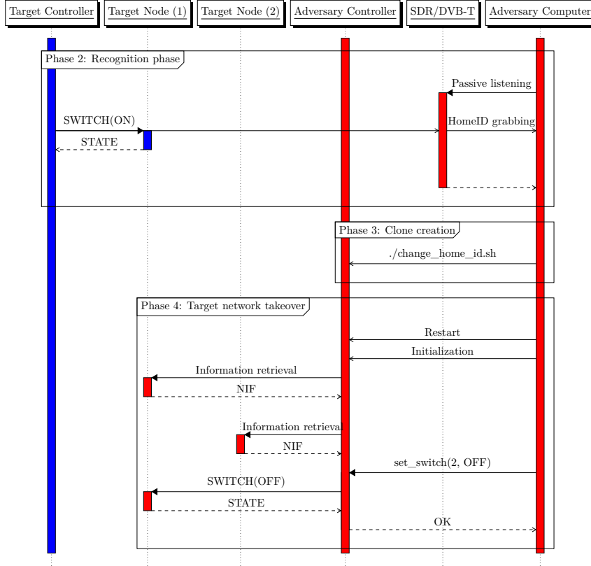
Figure 5: Attack phases
